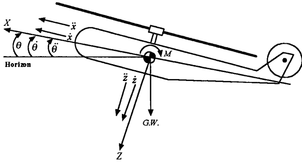
Fig. 5 Side view of helicopter's axis system.
