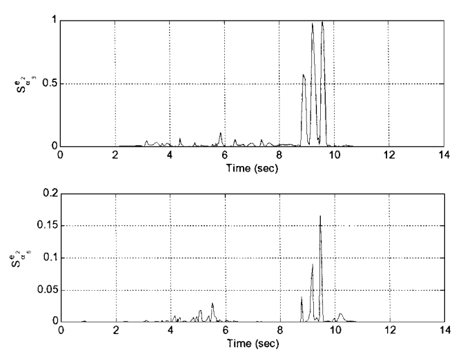
Fig. 13 Sensitivity of \dot{x} trajectory error with respect to \alpha_3 and \alpha_6 for the least-robust operation.
